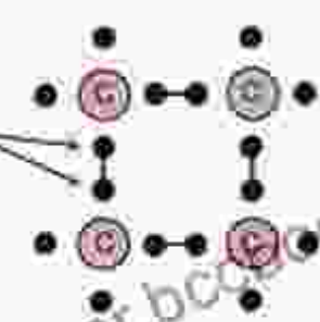
covalent bonding atoms share electrons
